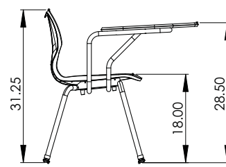
Flavors Rhombus Arm Chair Model 11825V Shown in Grey Mesh top with White edge and Apple Shell.
