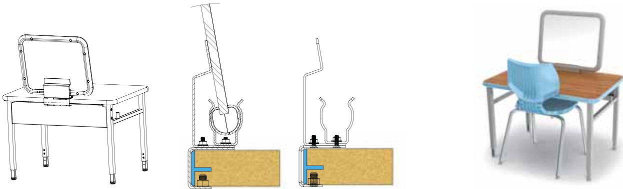
PRESENTup White Board, Model PU17700PLT shown with Clamp-on Desktop Bracket, Model PU17705PLT
