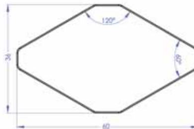
Two-Student Diamond Desk
