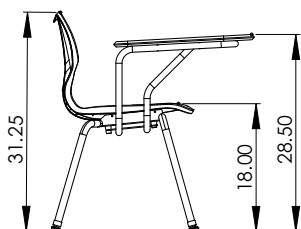
Flavors P-Tablet Arm Chair Model 11820V Shown in Grey Mesh top with Apple edge and Apple Shell.
