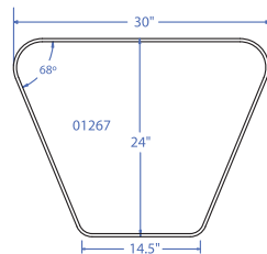
Huddle-8LS (top down view)
