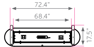
WALL STABILIZER
