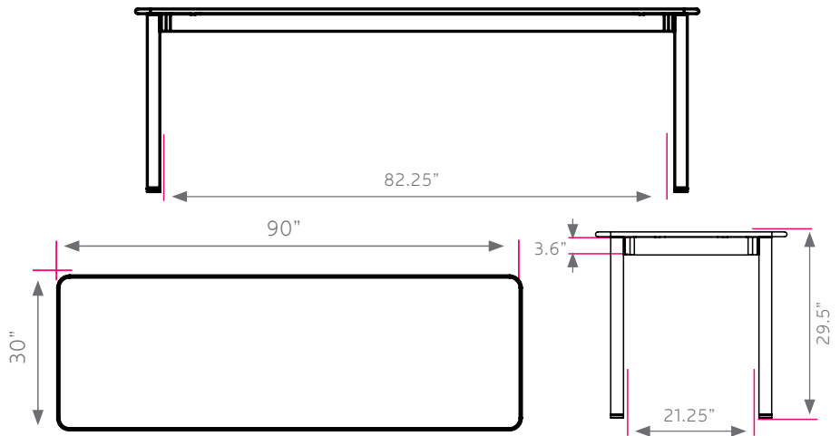
*XL2490, 24" x 90" UXL Rectangle Desk shown.
