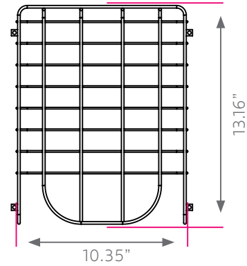
Outside Dimensions
