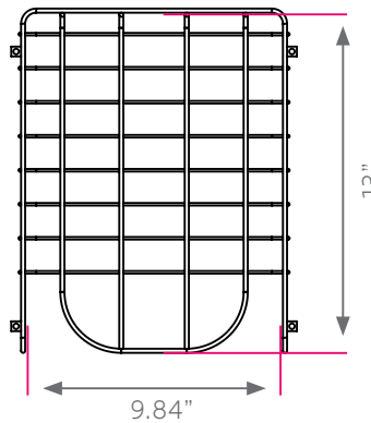
Inside Dimensions
