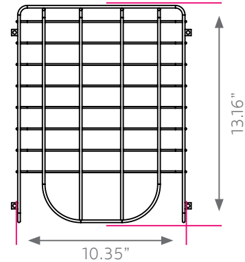
Outside Dimensions
