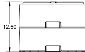
Height with rocker base disengaged
