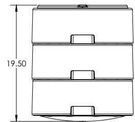
HEIGHT WITH ROCKER BASE ENGAGED (10° MOTION)
