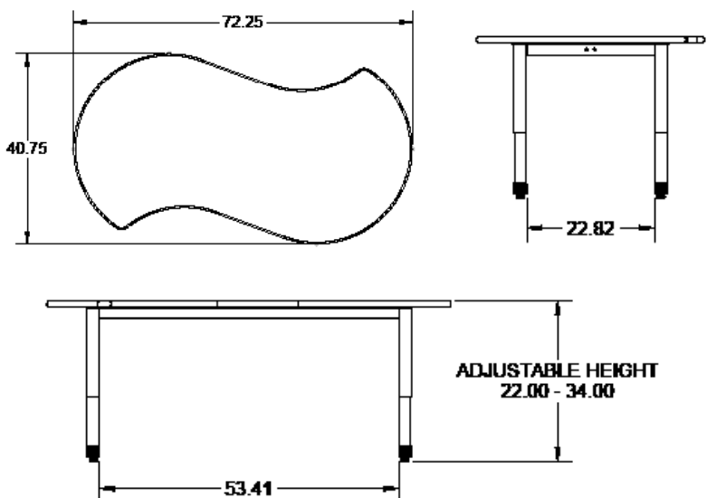
72" Interchange® Squiggle Table
