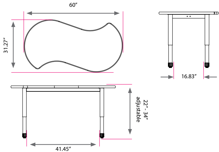
60" Interchange® Squiggle Table
