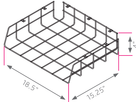
OUTSIDE DIMENSIONS
