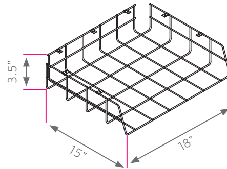
INSIDE DIMENSIONS
