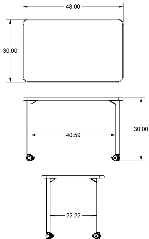
Drawings shown with 'EC' style legs, with optional 3" casters added.
