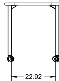
Drawings shown with 'EC' style legs, with optional 3" casters added.
