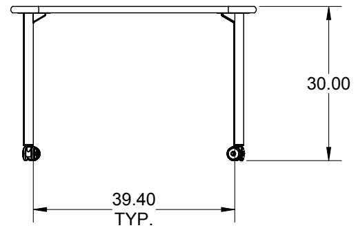
Drawings shown with 'EC' style legs, with optional 3" casters added.
