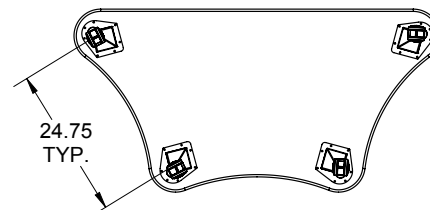
Drawings shown with 'EC' style legs, with optional 3" casters added.
