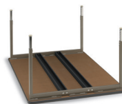
42" & 48" deep Models Two 2" x 3" 14-gauge steel support channels with 11-gauge steel endplates provide maximum stability.
