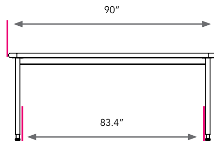
42" & 48" deep Models Two 2" x 3" 14-gauge steel support channels with 11-gauge steel endplates provide maximum stability.
