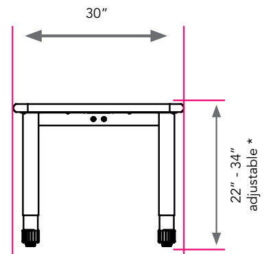
Center support channel is 2" by 3" wide 14-gauge steel, with 11-gauge steel endplates for maximum stability.
