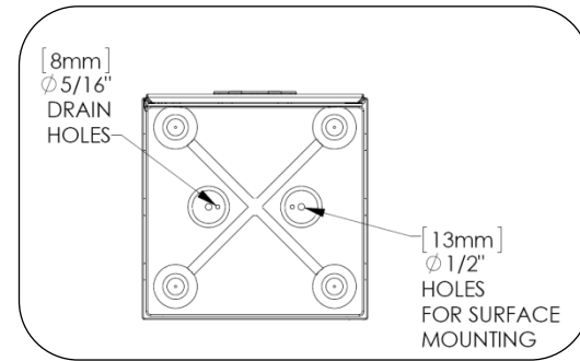
Fig. 1 – Bottom view of single unit base
