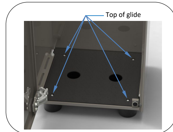
Fig. 2 – Base view showing tops of glides
